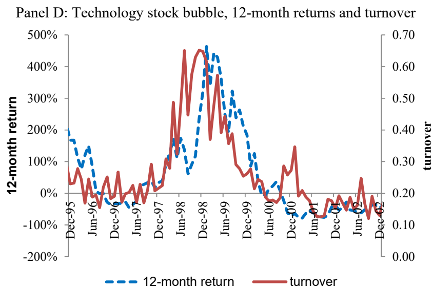
Fig. 6. Prices, returns, and volume during bubble episodes. Prices, past 12-month returns, and value-weighted turnover during four bubble episodes: utility stocks in 1929; technology stocks in 1998-2000; house prices in 2004-2006 as measured by the Case-Shiller 20-City Index; and oil in 2007-2008 as proxied by the price of the USO ETF. All data are monthly and value-weighted across stocks. For housing, turnover is measured as the number of existing-home sales.
